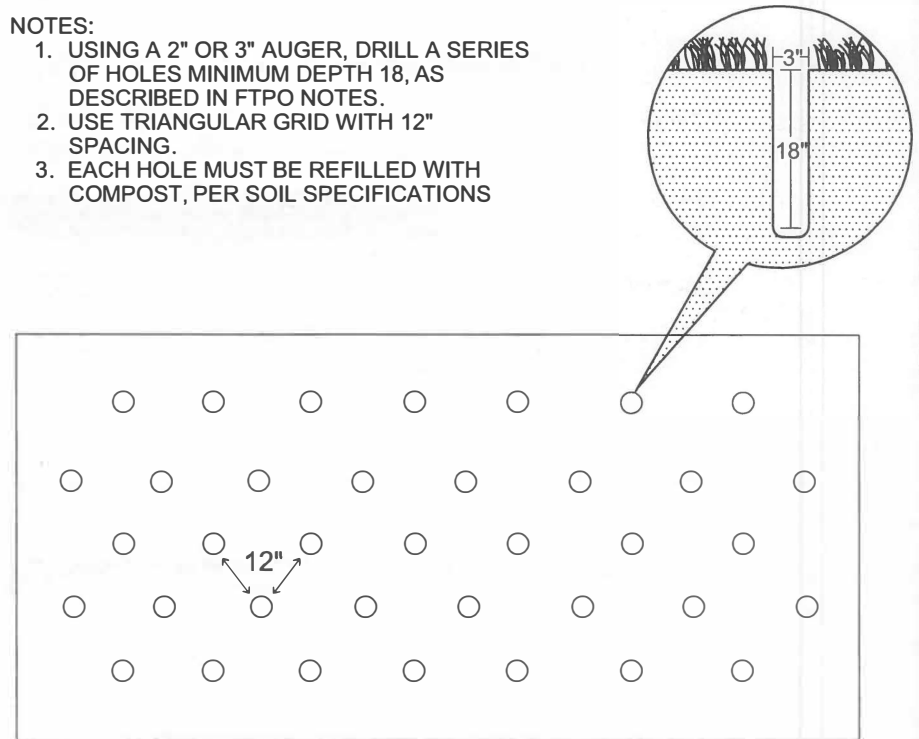
AERATION TO FULL EXTENT OF PLANTING BED
