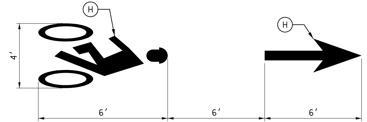
BICYCLE LANE PAVEMENT MARKING DETAIL SCALE: NOT TO SCALE
