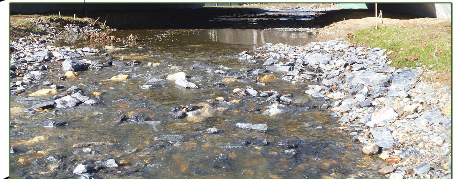
RIFFLE GRADE CONTROL EXAMPLE
