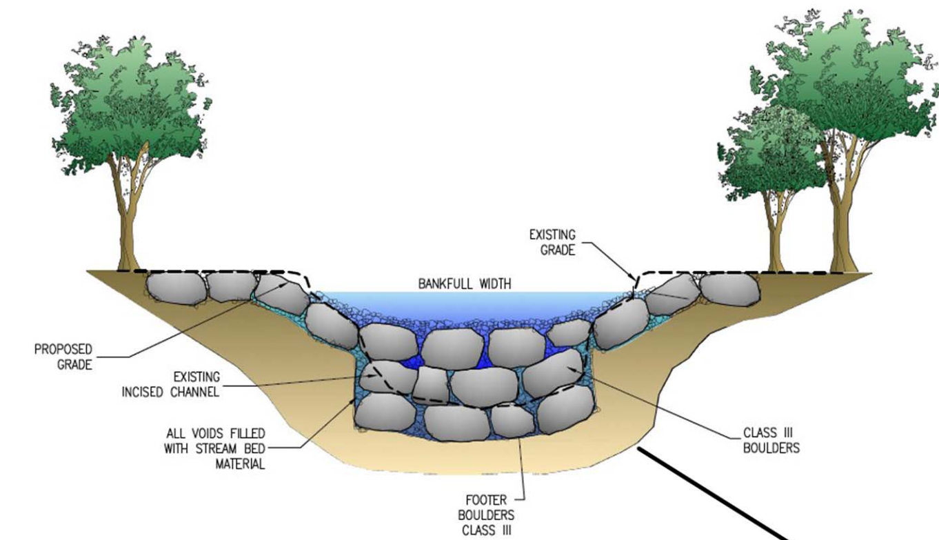
RIFFLE WEIR RENDERING
