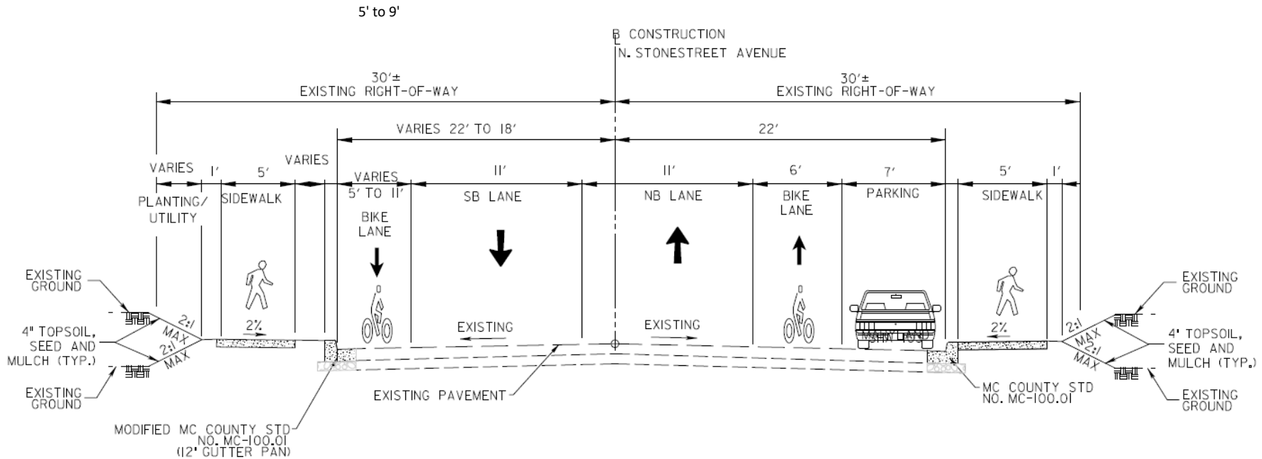
N. STONESTREET AVENUE – TYPICAL SECTION
